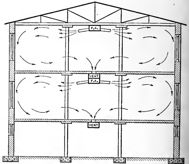
FIG. 4. ANOTHER ARRANGEMENT FOR BUILDINGS SEVERAL STORIES HIGH
